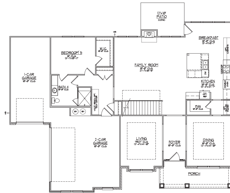
FIRST FLOOR PLAN - A
