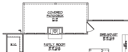
OPT LARGE COVERED PATIO FIRST FLOOR PLAN
