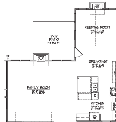
OPT. KEEPING ROOM FIRST FLOOR PLAN
