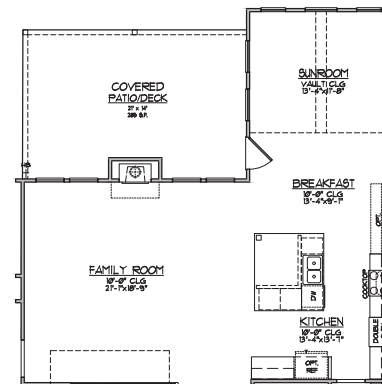
OPT SUNROOM & LARGE COVERED PATIO FIRST FLOOR PLAN
