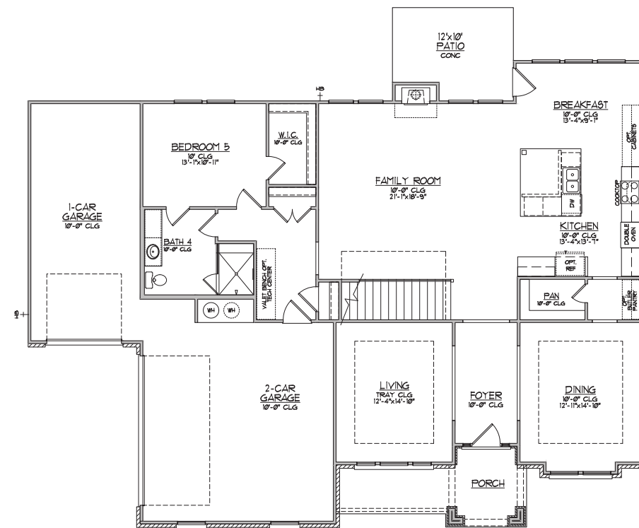
FIRST FLOOR PLAN - B
