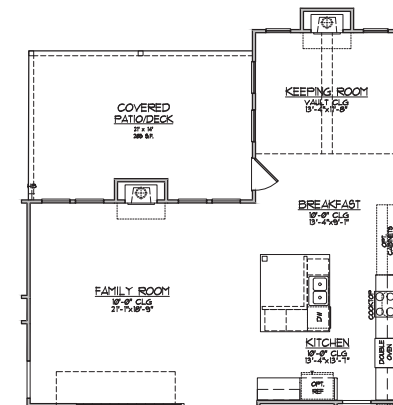
OPT. KEEPING ROOM & LARGE COVERED PATIO FIRST FLOOR PLAN
